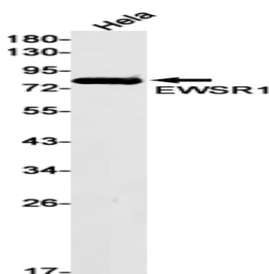
Western blot analysis of EWSR1 in HeLa lysates using EWSR1 antibody.
