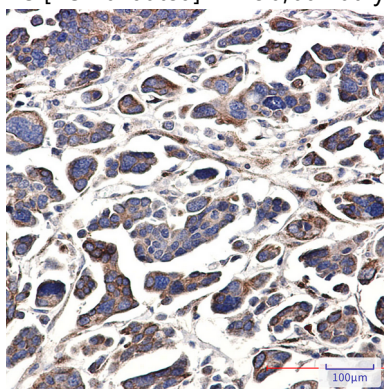
Immunohistochemistry analysis of paraffin-embedded Human Cholangiocarcinoma using G protein alpha 13 antibody. High-pressure and temperature Sodium Citrate pH 6.0 was used for antigen retrieval.
