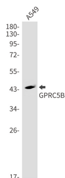
Western blot analysis of GPRC5B in A549 lysates using GPRC5B antibody.
