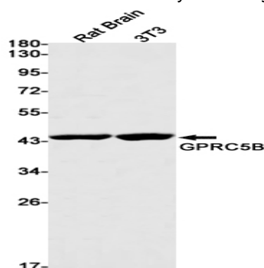
Western blot analysis of GPRC5B in rat Brain, 3T3 lysates using GPRC5B antibody.
