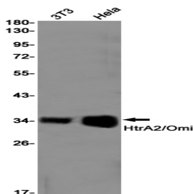
Western blot analysis of HtrA2/Omi in 3T3, HeLa lysates using HtrA2 antibody.
